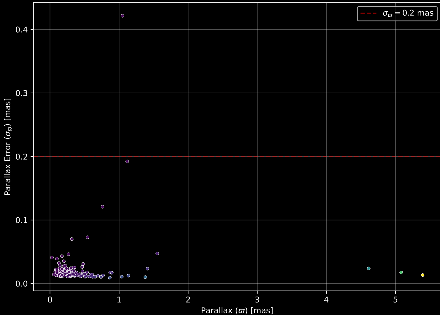
APOGEE DR17 Field: [Lac_1] Parallax Quality (n= 158)
