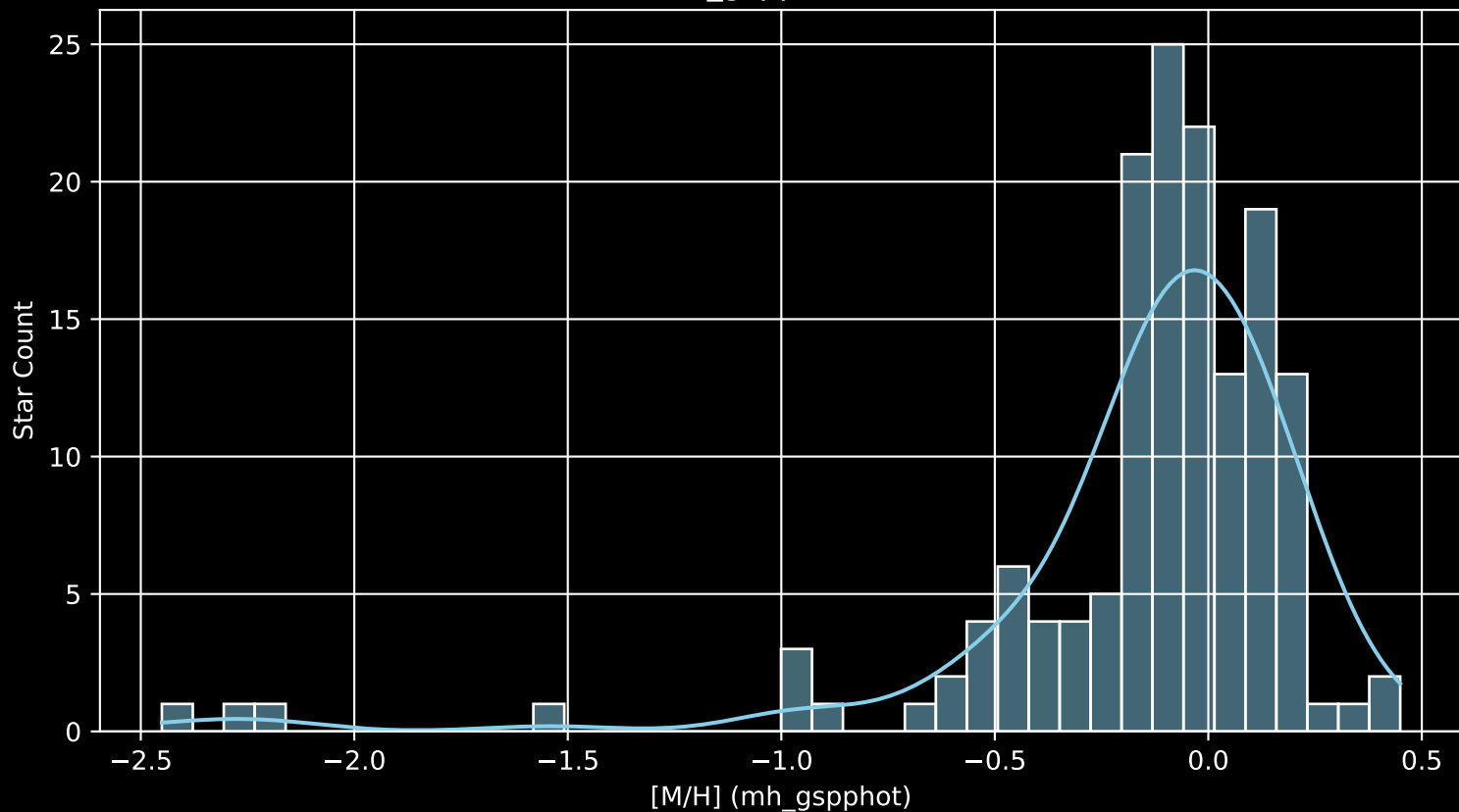
APOGEE DR17 Field: [Lac_1 [M/H] (mh_gspphot) (n= 151)
