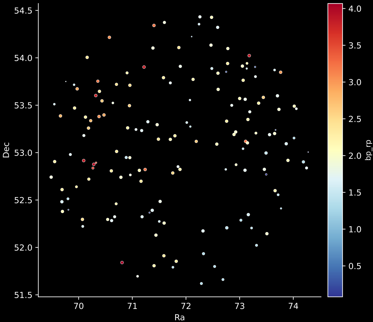
APOGEE DR17 Field: [Lac_1] Stars: 158
