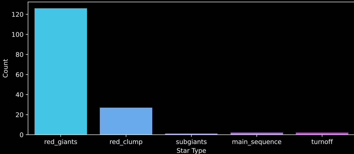
APOGEE DR17 Field: [Lac_1] Count plot of Star Type
